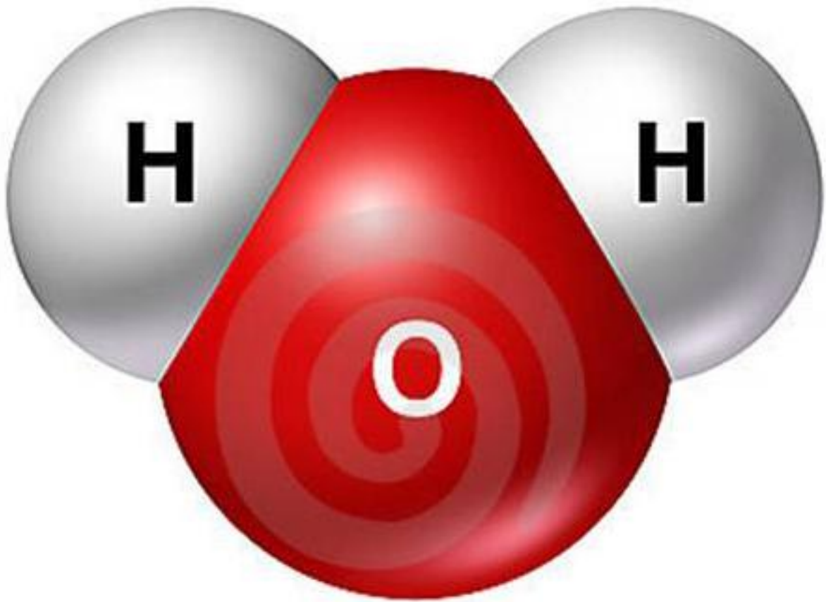
WATER MOLECULE
